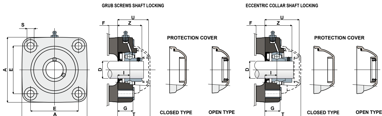
GRUB SCREWS SHAFT LOCKING
